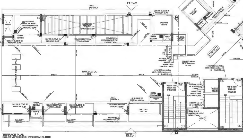
TERRACE PLAN 230 & 115 MM THICK BRICK WORK SHOWN AS ■
