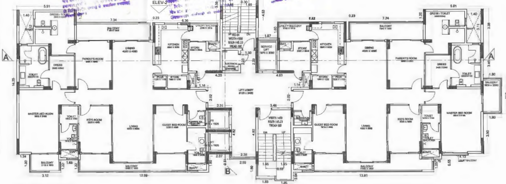
5TH, 8TH & 9TH FLOOR PLAN
